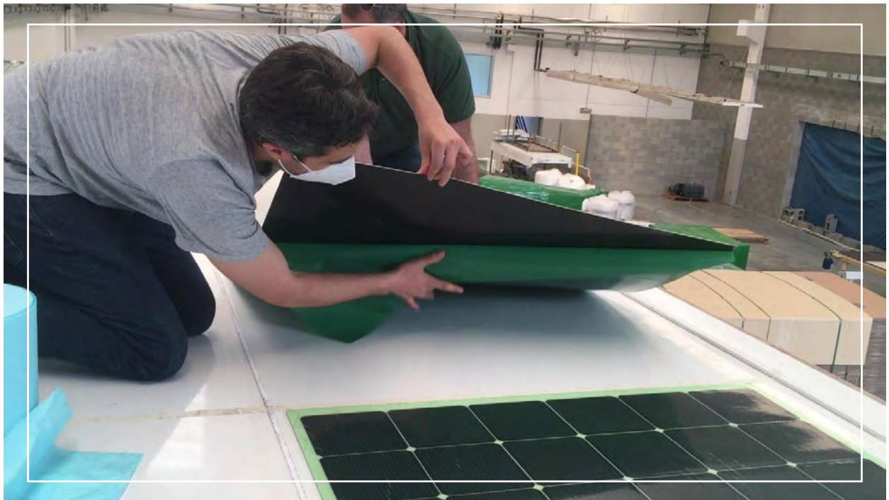
FIG. 7 Installation of flexible photovoltaic modules on the roof of a trailer. The protective film is removed from the rear adhesive before attachment.
